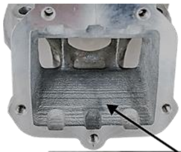
Single Core Cylinder showing linear structured cast surface finish:
